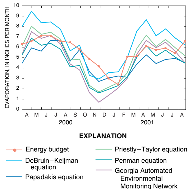
Figure 2. Comparison of monthly estimates of evaporation using empirical equations and the energy budget.
