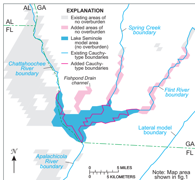
Figure 2. Boundary conditions of the digital ground-water model of the Upper Floridan aquifer in the Lake Seminole area showing modifications made to simulate preimpoundment conditions.
